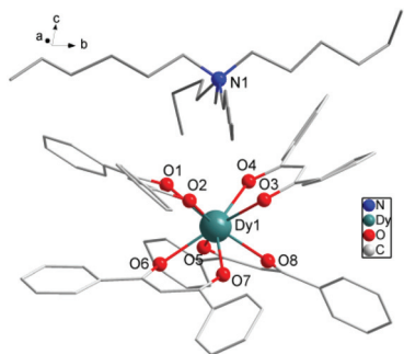
Fig. 1 Partially labelled molecular structure of [\text{Hex}_4\text{N}][\text{Dy}(\text{DBM})_4] , 1 . Colour code: Dy (teal), O (red), N (blue), C (grey). H atoms and disordered atoms were omitted for clarity.
