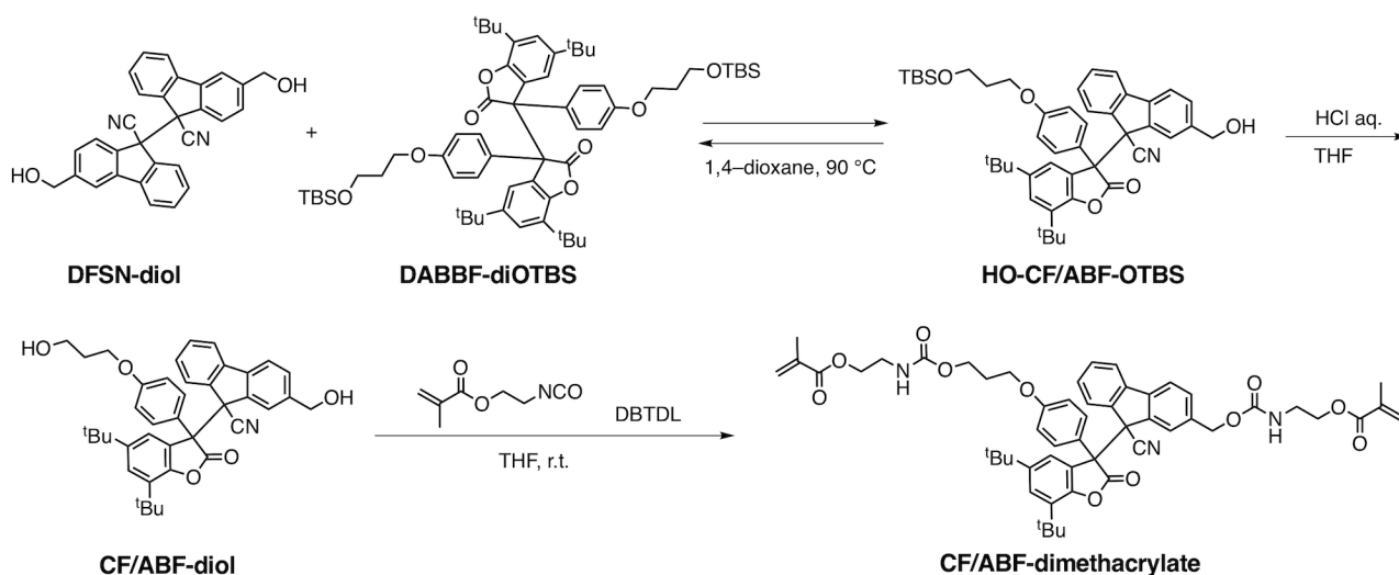
Scheme 1 Synthetic route of the CF/ABF cross-linker (CF/ABF-dimethacrylate).
