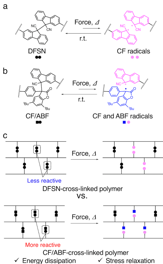
Fig. 1 (a) Equilibrium between DFSN and its radical species. (b) Equilibrium between CF/ABF and its radical species. Illustrations of (c) a DFSN-cross-linked polymer and a CF/ABF-cross-linked polymer, as well as the mechanism of energy dissipation and stress relaxation.
