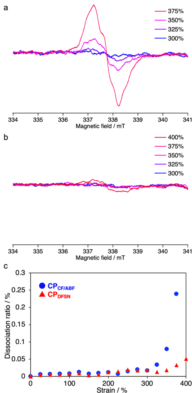
Fig. 6 EPR spectra of (a) \text{CP}_{\text{CF/ABF}} and (b) \text{CP}_{\text{DfSN}} at each strain (100 mm/min). Dissociation ratio of the CF/ABF and DFSN moieties of \text{CP}_{\text{CF/ABF}} and \text{CP}_{\text{DfSN}} at each strain.
