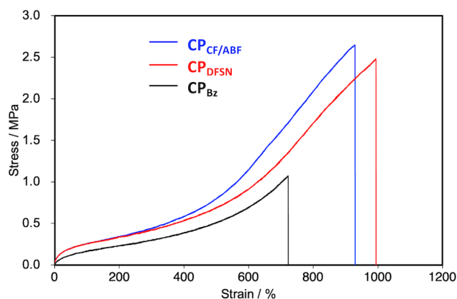
Fig. 5 Stress–strain curves of \text{CP}_{\text{CF/ABF}} (blue), \text{CP}_{\text{DfSN}} (red) and \text{CP}_{\text{Bz}} (black) films (100 mm/min, 30 °C).
