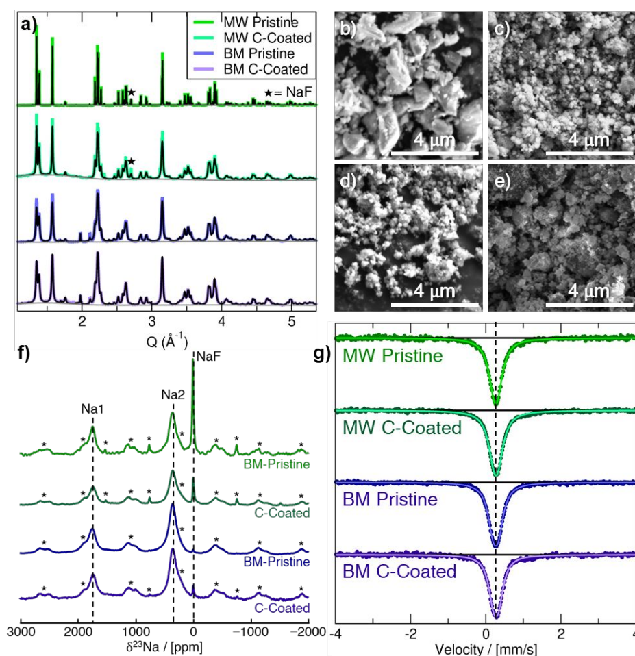
Figure 1, Structural Characterization of As-Prepared \text{Na}_3\text{FeF}_6 Materials. a) SXR pattern and Rietveld refinement (black) for each sample. b-e) SEM images obtained of MW pristine (b), MW C-coated (c), BM pristine (d), and BM C-coated (e) samples. f) ^{23}\text{Na} spin echo NMR spectra collected on the as-prepared materials. Each spectrum is scaled according to the number of moles of material in the rotor and the number of scans collected during the experiment. Spinning sidebands are indicated by an asterisk (*). g) Zero-field, 298 K ^{57}\text{Fe} Mössbauer spectra obtained on the as-prepared materials. The dashed line corresponds to an isomer shift ( \delta ) of 0.27 mm/s typical of an \text{Fe}^{3+} ion in an octahedral environment.
