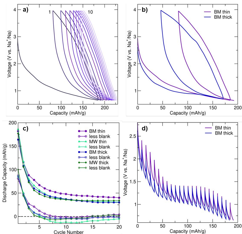
Figure 2, Electrochemical Characterization of \text{Na}_3\text{FeF}_6 . a) First ten cycles for BM- \text{Na}_3\text{FeF}_6 thin cells ( C/20 rate). b) First two charge and discharge cycles for BM- \text{Na}_3\text{FeF}_6 thin and thick cells ( C/20 rate). c) Discharge capacity retention for \text{Na}_3\text{FeF}_6 cells (filled symbols) and for \text{Na}_3\text{FeF}_6 cells with the corresponding blank cell capacity subtracted (unfilled symbols). Three cells were averaged for each point. d) GITT test ( C/20 rate) for the first discharge cycle of BM thin and thick cells.
