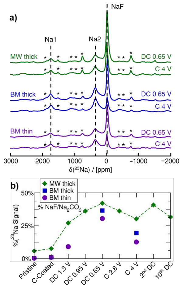
Figure 3, 23 Na NMR of ex situ Na 3 FeF 6 . a) 23 Na spin echo NMR spectra of ex situ Na 3 FeF 6 with each spectra scaled according to number of moles of material in the rotor and the number of scans used in the experiment. Spinning sidebands are indicated by an asterisk (*). b) Percent of the 23 Na signal ( \pm 5\% ) after accounting for signal relaxation over the course of the NMR measurement ( T_2' losses) corresponding to diamagnetic NaF at various states of charge.
