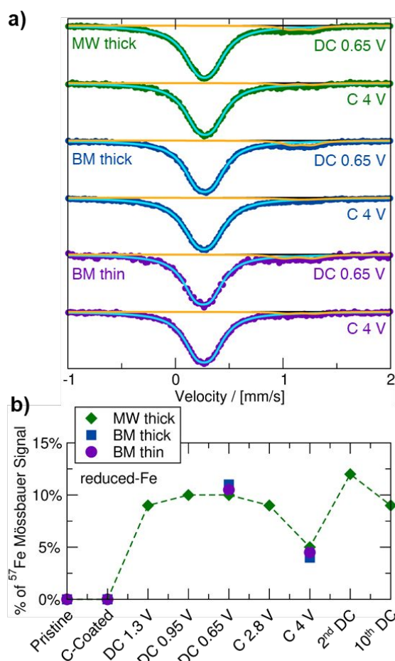
Figure 4, ^{57}\text{Fe} Mössbauer of ex situ \text{Na}_3\text{FeF}_6 . a) ^{57}\text{Fe} Mössbauer spectra of ex situ \text{Na}_3\text{FeF}_6 fit with two doublets for O_h\text{-Fe}^{3+} and reduced-Fe. b) Change in the amount of ^{57}\text{Fe} signal ( \pm 2\% ) corresponding to the O_h\text{-Fe}^{3+} and reduced-Fe species at different states of charge.
