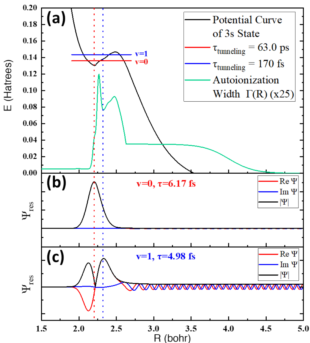
Figure 6. Vibrational dynamics on the calculated 3s Rydberg potential curve whose imaginary part is given by the R -dependent electronic autoionization width in the local complex potential, E_{\text{res}}(R) - i\Gamma(R)/2 . (a) Potential curve E_{\text{res}}(R) , width \Gamma(R) , and location of tunneling vibrational levels, (b) the v=0 vibrational wave function, and (c) the v=1 vibrational wave function showing tunneling into the dissociative region of the potential. Red and blue vertical dashed lines mark the location of the maxima in the absolute value of the vibrational wave functions of v=0 and v=1 , respectively.
