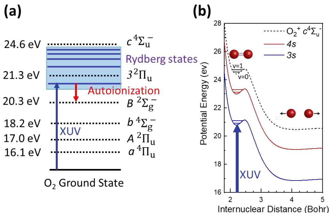
Figure 1. (a) Energy level diagram of O_2^+ states and Rydberg states converging to O_2^+ c^4\Sigma_u^- state. Dashed lines are ionic states and solid lines are neutral Rydberg states.
