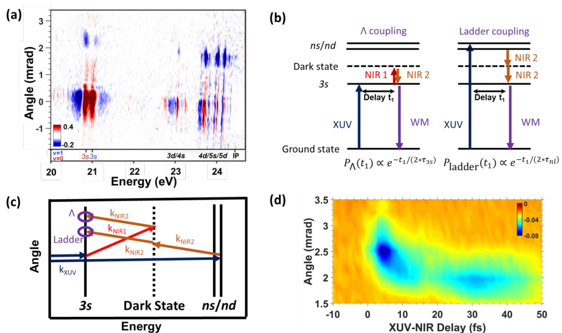
Figure 4. (a) Camera image at the overlap of all three pulses. Positive (red) features represent absorption while negative (blue) features represent emission. Spatially-isolated wave-mixing signals are observed around 1.5~2.8 mrad. (b) Two possible pathways to generate wave-mixing (WM) signals from the 3s state. (c) Phase matching conditions and the emission angles of \Lambda -type coupling and ladder-type coupling (d) Angle-dependent transient wave-mixing signals of v=0 level (20.85 eV) of the 3s Rydberg state. The component around 2.5 mrad corresponds to \Lambda -type coupling from 3s Rydberg state itself while the component around 2.0 mrad corresponds to ladder-type coupling from higher n Rydberg states.
