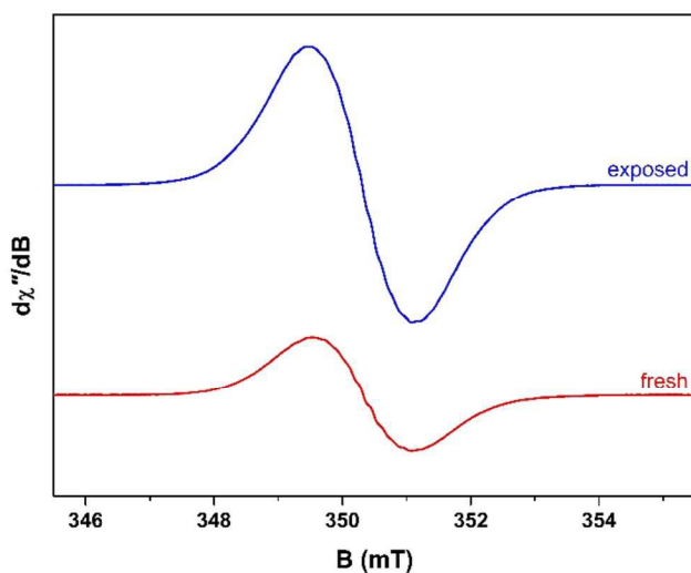
Fig. 2 Comparison of the X-band EPR spectra for the fresh (red) and air-exposed (blue) catalyst recorded at ambient temperature on an aliquot collected after 2 h TOS with 20% MeOH/Ar at reaction temperature 260 °C.
