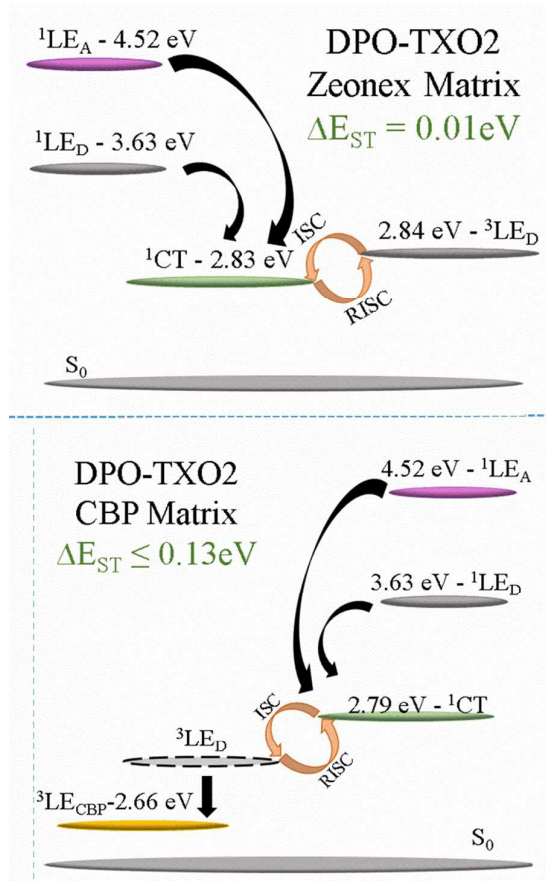
Fig. 11 Energy levels diagram describing the excited dynamics of DPO-TXO2 in zeonex and CBP matrix, evidencing the localized and charge transfer states.
