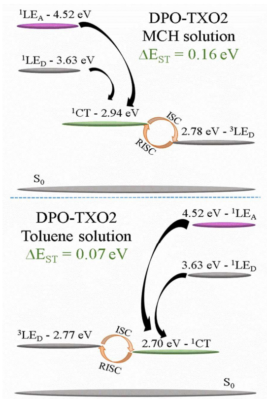
Fig. 7 Energy levels diagram describing the excited dynamics of DPO-TXO2 in Toluene and MCH solutions, evidencing the localized and charge transfer states.
