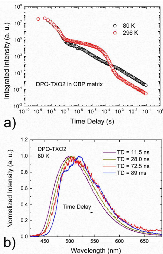
Fig. 10 a) Time resolved fluorescence decay of DPO-TXO2 in CBP matrix. The curves were obtained with 355 nm excitation. b) Time resolved normalized emission spectra in the entire region of analyses.
