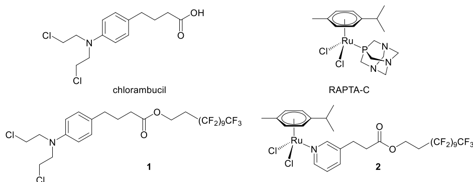
Figure 1. Chemical structures of chlorambucil, RAPTA-C and the thermoactive derivatives 1 and 2 .
