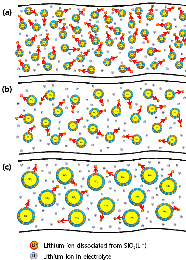
Fig. 10. Schematic presentation of \text{Li}^+ ion transport in composite polymer electrolytes containing core-shell structured \text{SiO}_2(\text{Li}^+) particles with core diameters of (a) 250 nm, (b) 420 nm and (c) 810 nm.
