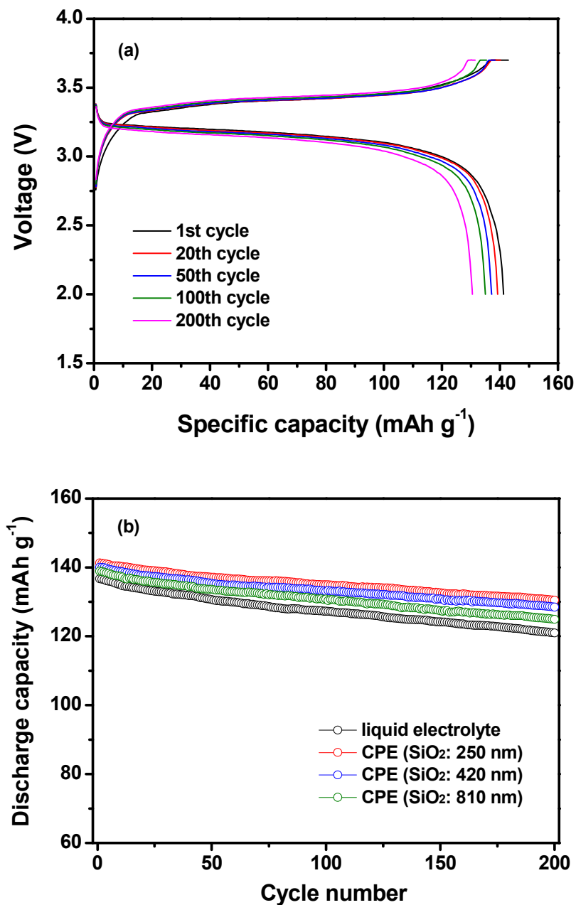
Fig. 8. (a) Charge and discharge curves of a lithium-ion polymer cell assembled with composite polymer electrolyte containing SiO 2 (Li + ) particles with a core diameter of 250 nm (0.5C CC and CV charge, 0.5C CC discharge, cut-off: 2.0-3.7 V), and (b) discharge capacities of lithium-ion polymer cells assembled with different electrolytes. CPE refers to composite polymer electrolyte.
