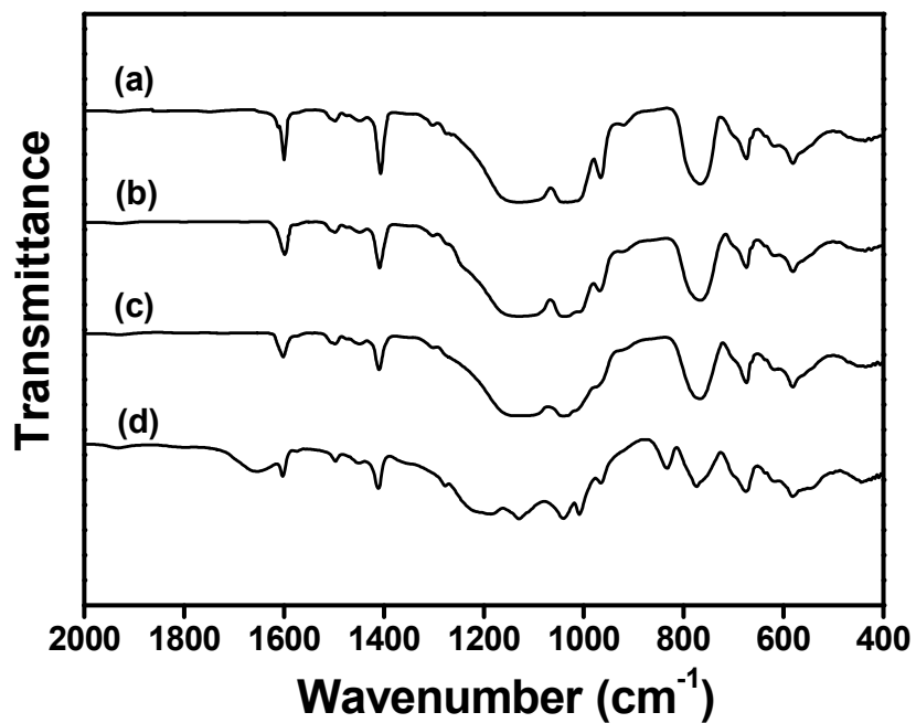
Fig. 3. FT-IR spectra of SiO 2 core particles with an average diameter of (a) 250 nm, (b) 420 nm, (c) 810 nm and (d) core-shell structured SO 2 particles (core size: 250 nm) encapsulated by poly(sodium 4-styrenesulfonate).
