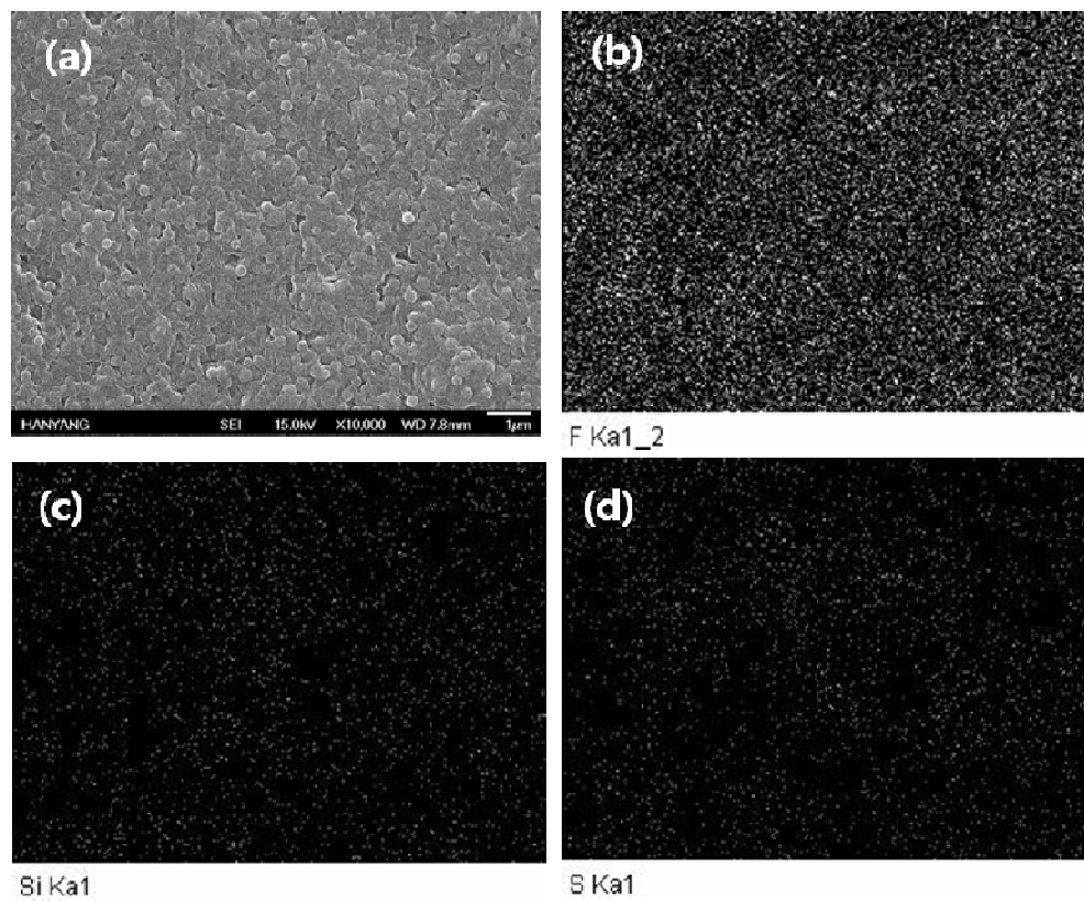
Fig. 5. (a) SEM image and EDAX mapping images of (b) fluorine, (c) silicon and (d) sulfur in the composite polymer membrane containing 20 wt% core-shell structured \text{SiO}_2(\text{Li}^+) particles with a core diameter of 250 nm.
