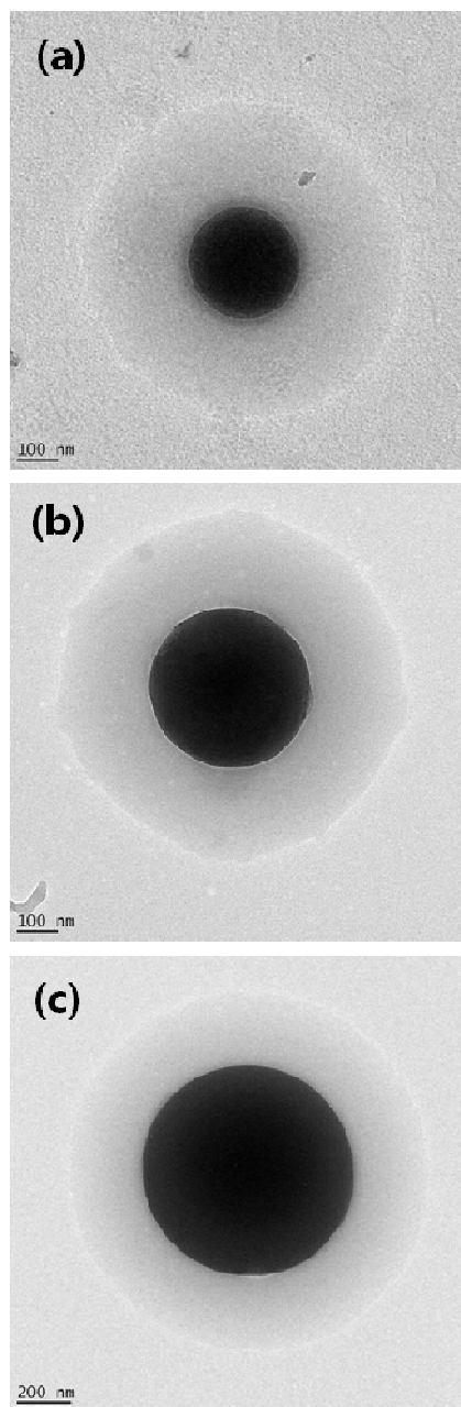
Fig. 4. TEM images of core-shell structured SiO 2 particles with core diameters of (a) 250 nm, (b) 420 nm and (c) 810 nm.
