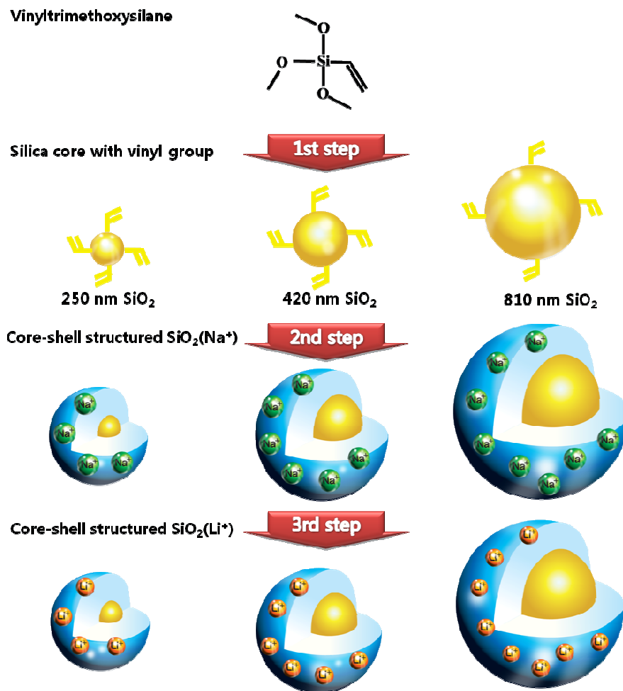
Fig. 1. Schematic reaction scheme for synthesis of core-shell structured SiO 2 (Li + ) particles with different core diameters.
