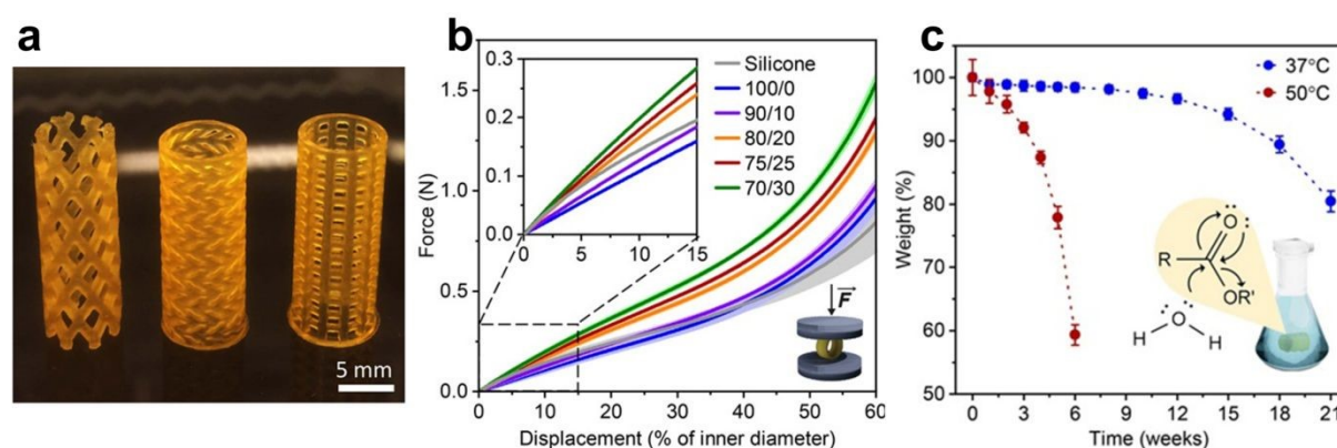
Figure 4. (a) 3D-printed biodegradable stents with different designs. (b) Force-displacement curves of dual-polymer stents with different ratio and a NOVATECH silicone stent. (c).
