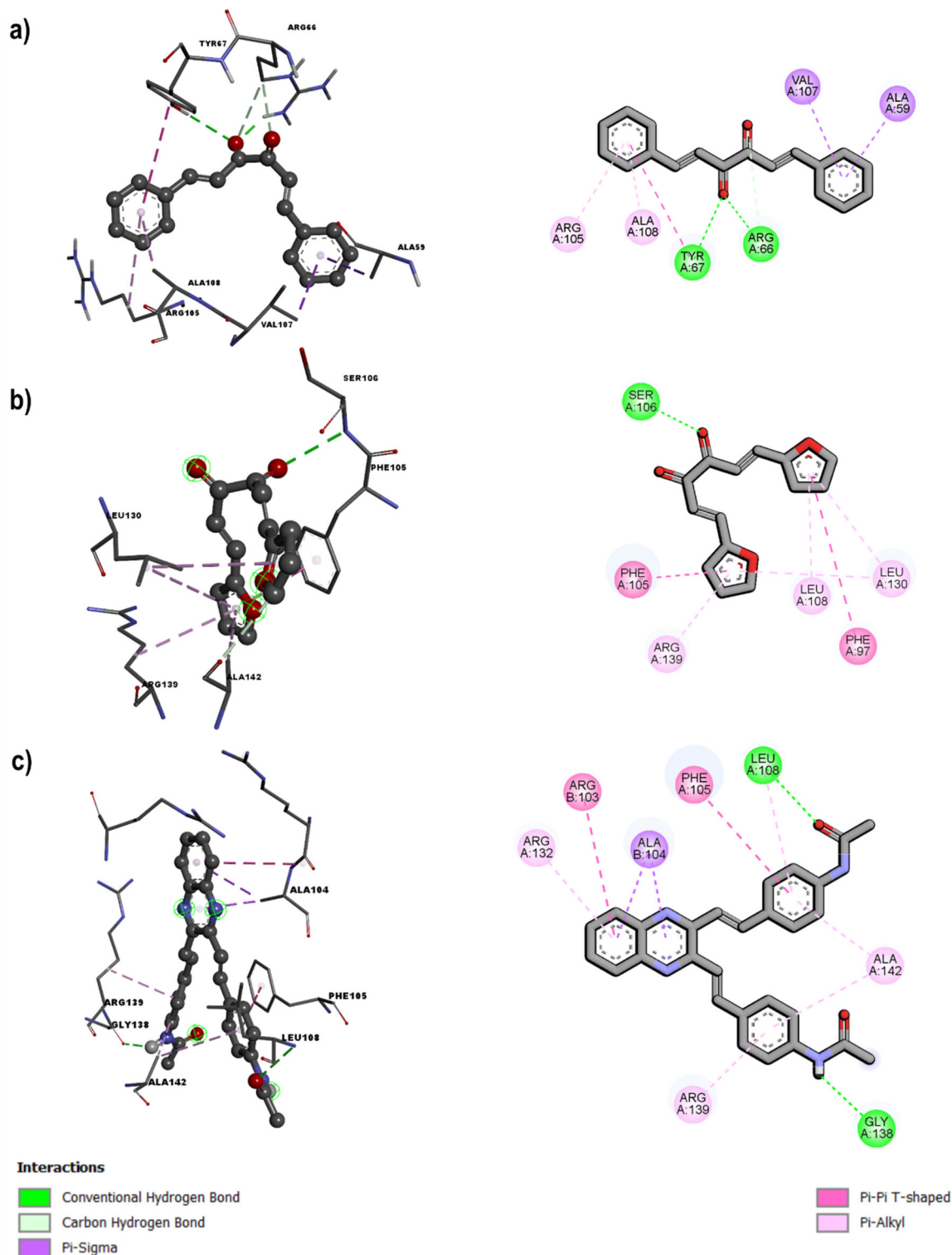
Fig. 2 3D and 2D pictures of (a) compound M1 at the active site of Bcl-2 protein, (b) M3 complexed with the active site of Bcl-xl and (c) compound M5 bound to the binding site of Bcl-2.
