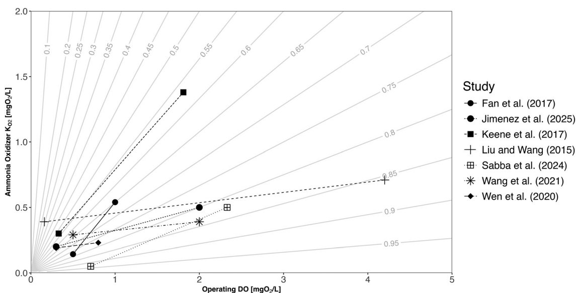
Fig. 3 Ammonia oxidation capacity contour plot showing relative ammonia oxidation rate for different values of operating DO and ammonia oxidizer K_{O_2} . Relative ammonia oxidation rate assumes all else is held equal and is calculated via the Monod function ( S_{O_2}/(K_{O_2} + S_{O_2}) ) where S_{O_2} is the operating DO. Gray lines indicate equal-rate contours, i.e. all combinations of operating DO and ammonia oxidizer K_{O_2} that fall along a contour will give the same relative ammonia oxidation rate. When operating DO is reduced, ammonia oxidizer K_{O_2} must also reduce along a slope parallel the nearest line, or ammonia oxidation capacity will be different at the lower operating DO. Experimental findings where estimates of ammonia oxidizer K_{O_2} was reported at different operating DO are shown on the plot. Slopes less than the slope of surrounding contours indicate a loss of capacity, greater slopes a gain of capacity (the more significant the deviation, the greater the relative loss or gain in capacity). Studies included in this figure are only those that specifically reported both high and low operating DO values and ammonia oxidizer K_{O_2} .
