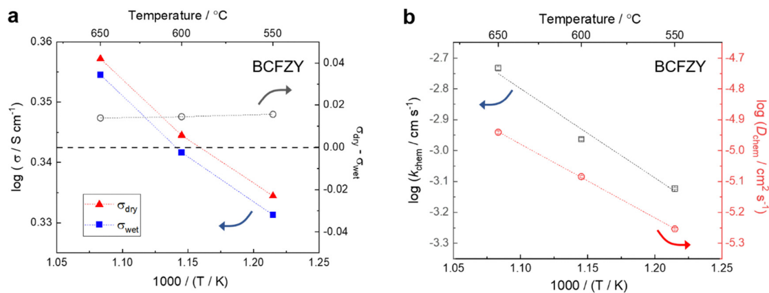
Fig. 4 (a) Electrical conductivity of BCFZY under dry and 3% \text{H}_2\text{O} -humidified atmosphere ( p_{\text{O}_2} = 0.156 atm) at various temperatures. The conductivity decreases under humidified conditions, providing the evidence of hydrogenation behavior. (b) Surface exchange coefficient ( k_{\text{chem}} ) and chemical diffusion coefficient ( D_{\text{chem}} ) of BCFZY as a function of temperature, extracted by fitting ECR data obtained during dehydrogenation.
