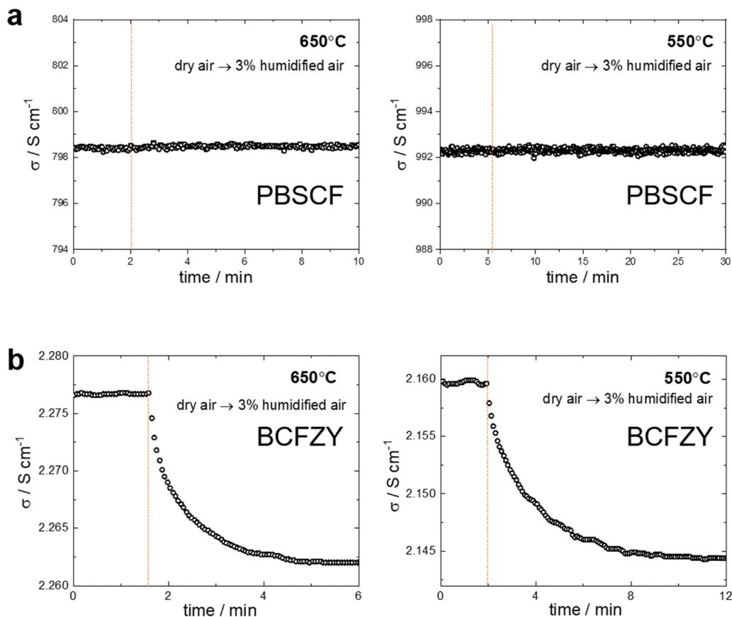
Fig. 3 Conductivity response of PBSCF and BCFZY samples under gas switching from dry to 3% \text{H}_2\text{O} -humidified atmosphere (indicated by the red line) at 650 °C and 550 °C. (a) PBSCF ( p_{\text{O}_2} = 0.17 atm), showing negligible change in conductivity upon proton uptake (b) BCFZY ( p_{\text{O}_2} = 0.156 atm), exhibiting a clear decrease in conductivity upon proton uptake.
