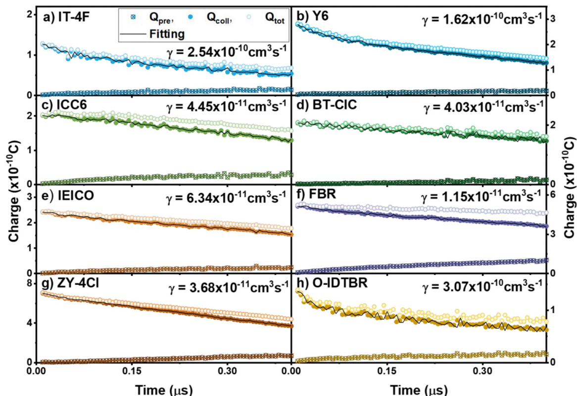
Fig. 7 Charge recombination in P3HT:NFA devices measured by time-delayed collection field experiments. (a) P3HT:IT-4F, (b) P3HT:Y6, (c) P3HT:ICC6, (d) P3HT:BT-CIC, (e) P3HT:IEICO, (f) P3HT:FBR, (g) P3HT:ZY-4Cl and (h) P3HT:O-IDTBR. Where, ( Q_{pre} ) is the amount of charge extracted during pre-bias, and ( Q_{coll} ) is the amount of charge extracted during collection bias ( V_{coll} = -4 V) and their fits as a function of delay time between excitation and the beginning of extraction yields the bi-molecular recombination rate ( \gamma ). Thus, the total extracted charges Q_{tot} = Q_{pre} + Q_{coll} .
