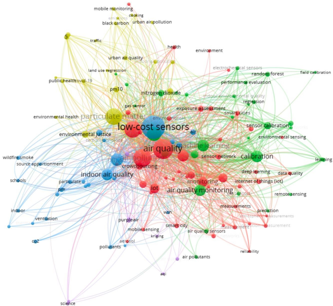
Figure 6: A keyword co-occurrence network showing relationships and thematic clusters between low-cost sensors and key concepts in air quality monitoring.
