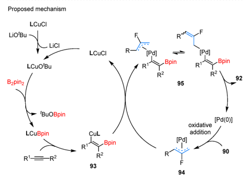
Scheme 22 Catalytic cis -borylfluoroallylation of alkynes.
