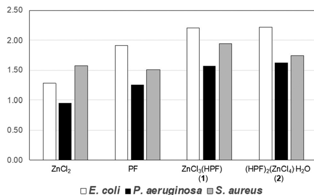
Fig. 6 Relative antimicrobial activities of proflavine, ZnCl 3 (HPF), and (HPF) 2 (ZnCl 4 )·H 2 O normalized to the activity of AgNO 3 (value of 1.00 corresponds to silver nitrate efficacy). Reproduced from ref. 109.
