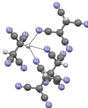
Fig. 3 Fragment of the crystal structure of 1,1,2,2-ethanetetracarbonitrile (BUGKIX01 ref code). 82 The H \cdots N intermolecular contacts are designated by the black narrow lines.
