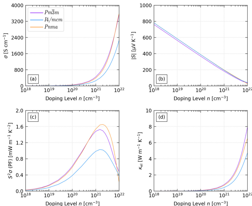
Fig. 7 Predicted scalar-average electrical properties of n-type Pm\bar{3}m , I4/mcm and Pnma \text{SrTiO}_3 as a function of extrinsic carrier concentration n ("doping level") at a fixed temperature T = 1000 K: (a) electrical conductivity \sigma , (b) absolute Seebeck coefficient |S| , (c) power factor S^2\sigma (PF), and (d) electronic thermal conductivity \kappa_{\text{el}} .
