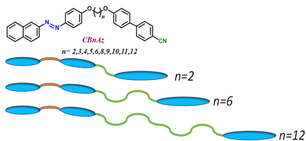
Fig. 15 Cartoon diagram showing the distribution of spacer length along with the chemical structure.
