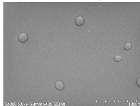
Fig. 9 SEM image of \text{Al}_2\text{O}_3 film after exposure to \text{NbCl}_5 at 350 °C.
