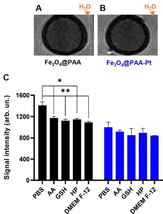
Fig. 4 T_2 -weighted phantom image of (A) Fe 3 O 4 @PAA and (B) Fe 3 O 4 @PAA-Pt(IV) nanoparticles (455 μM of Fe) in PBS, surrounded by water, at 3.0 T. (C) T_2 -weighted MR signals of Fe 3 O 4 @PAA (black, 200 μM of Fe) and Fe 3 O 4 @PAA-Pt(IV) nanoparticles (blue, 200 μM of Fe) in the presence of 100 μM of ascorbic acid (AA), glutathione (GSH), hydrogen peroxide (HP), and DMEM F-12 medium, at 3.0 T, * p < 0.035, ** p < 0.02. Error bars indicate standard deviation (SD).
