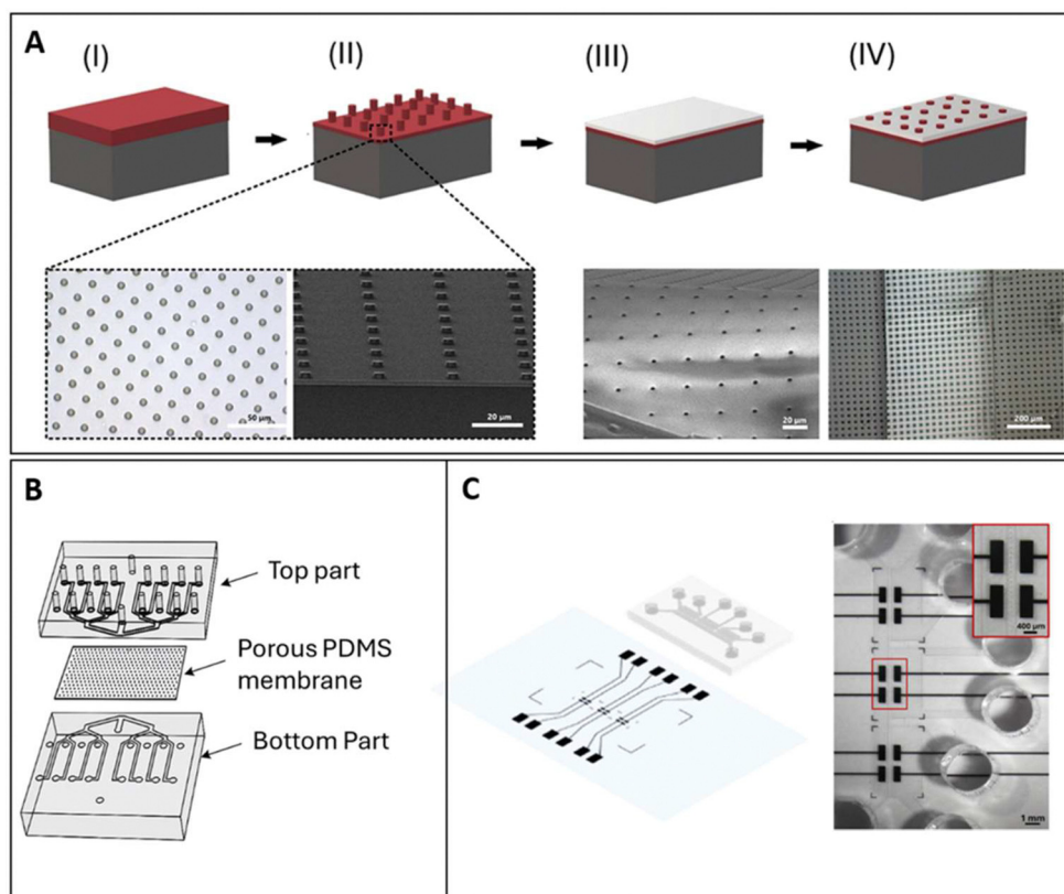
Fig. 8 (A) Graphical scheme for the thin PDMS membrane fabrication process via photolithographic technique. Left blow-up: top and side views of the photoresist columns; right blow-up: images of the PDMS membrane. (B) Scheme of the final device assembly with the PDMS membrane embedded between the two-layer microfluidic device. (C) Left: rendering of the microfluidic device and the glass coverslip with the electrodes scheme. Right: optical image of the fabricated device with the PDMS chip bonded onto the electrode layer. Reproduced from Ref. Zakharova and Ceccarelli with permission from the Royal Society of Chemistry.
