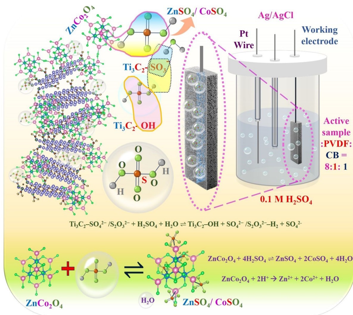
Fig. 4 Illustration of the redox-mediated interactions occurring within the \text{SO}_4^{2-} / \text{S}_2\text{O}_3^{2-} ions present in TS integrated with \text{ZnCo}_2\text{O}_4 in \text{H}_2\text{SO}_4 aqueous electrolyte.
