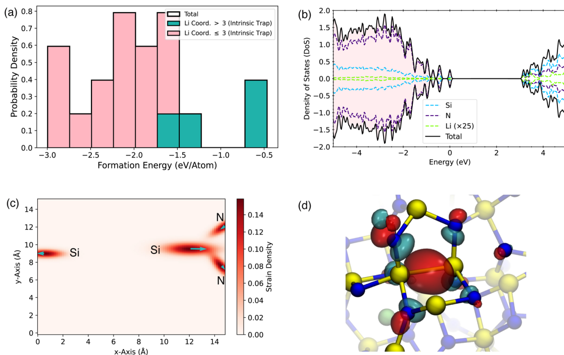
Fig. 4 (a) Distribution of \text{Li}_2 formation energies in \text{a-Si}_3\text{N}_4 . As in Fig. 2a, the total distribution (black outline) is subdivided based on coordination and trapping site. Histogram bars represent the probability–density estimate p(x) = \frac{n_i}{N\Delta x} ; the distribution is normalised by \int p(x) dx = 1 . (b) DoS showing the occupied bi-polaron state, the filled states are indicated by the shaded region below the Fermi energy. For clarity the Li peak has been increased by a factor of 25. (c) Average 2D projection of the strain induced as a result of \text{Li}_2 incorporation and the associated bi-polaron formation. (d) Doubly occupied bi-polaron state forming a Si–Si bond with a length of 2.32 Å. Blue spheres shows nitrogen, and yellow silicon. Red iso-surface shows the spin up channel, and light blue the spin down channel.
