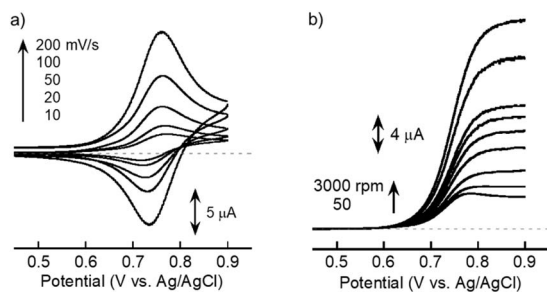
Fig. 3 Voltammetric responses obtained for 2 mM P1 dissolved in the aqueous electrolyte. (a) Cyclic voltammograms scanned at 10, 20, 50, 100, and 200 mV s -1 . (b) Hydrodynamic voltammograms. The electrode disk was rotated at 50, 100, 200, 400, 600, 1000, 2000, and 3000 rpm.
