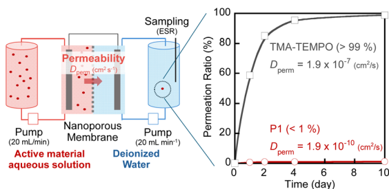
Fig. 4 Configuration of the cell for the permeation test and the related experimental result. The active materials were flowed at 20 mL min -1 to proceed with permeation to the other cell with only water.
