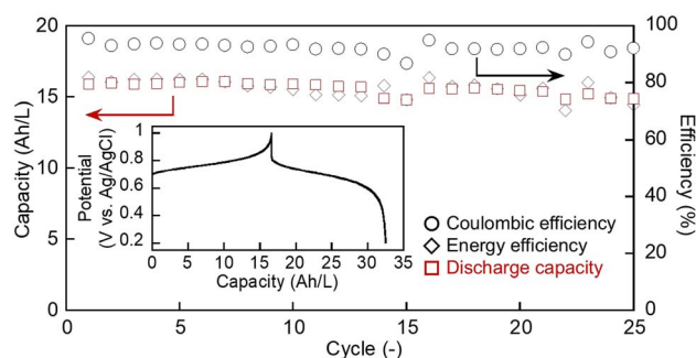
Fig. 5 Cycle performance of the prototype RFB with 0.25 C, 20 Ah L -1 (0.75 M). Inset: charge–discharge curves of the 1st cycle.
