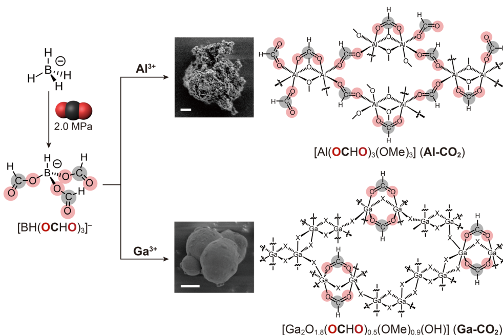
Fig. 1 Schematic illustration of the synthesis and proposed structures of \text{M-CO}_2 ( \text{M} = \text{Al}^{3+}, \text{Ga}^{3+} ). Carbon and oxygen atoms derived from \text{CO}_2 are highlighted. The symbol X in the structure of \text{Ga-CO}_2 indicates either \text{O}^{2-} , \text{OH}^- , or \text{OMe}^- . SEM images of \text{M-CO}_2 are displayed, respectively. The scale bar indicates 1 \mu\text{m} .
