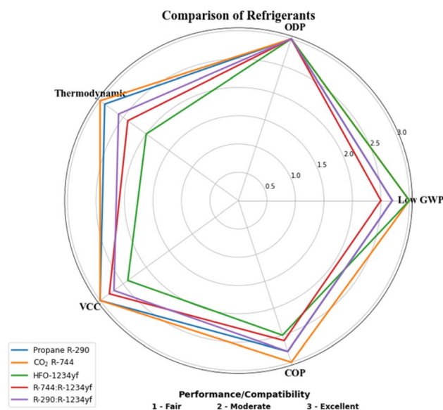
Fig. 7 Comparison of the thermodynamic, technical and environmental compatibility of propane, CO 2 , propane + R1234yf and CO 2 + R1234yf blends.
