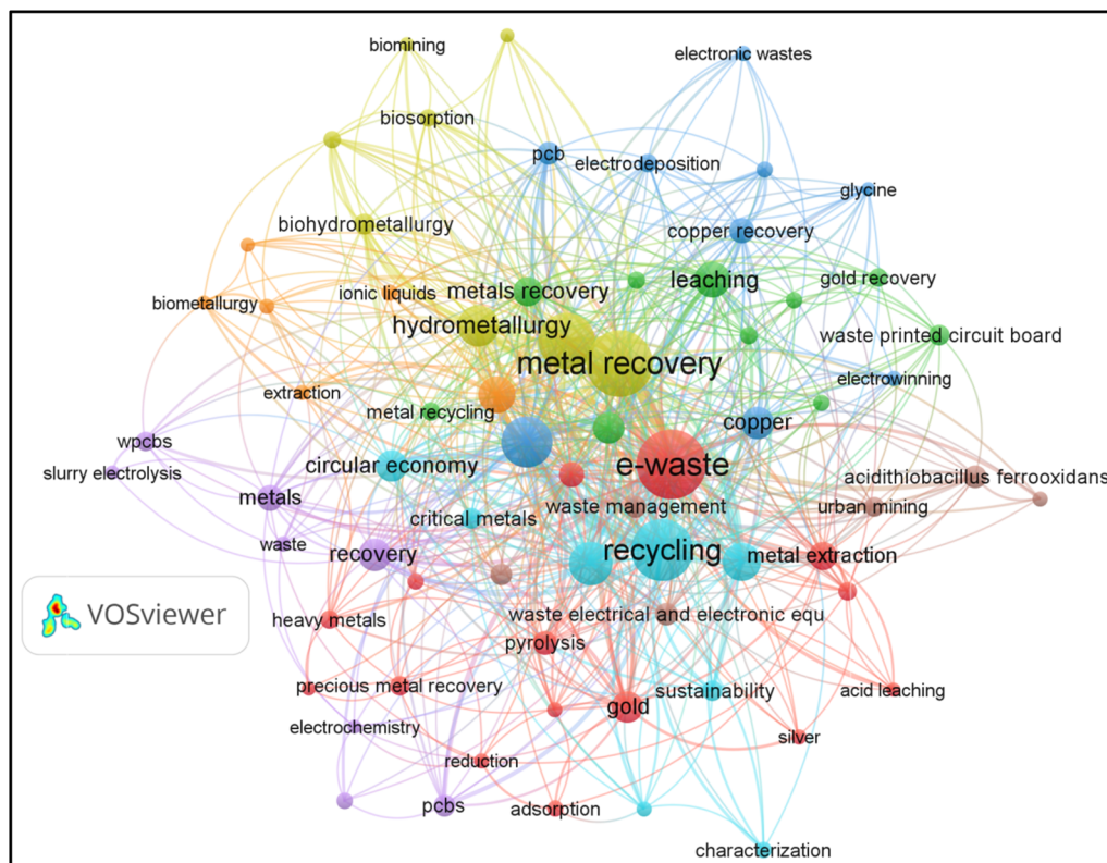
Fig. 6 Network diagram showing major keywords for metal recovery in e-waste management.
