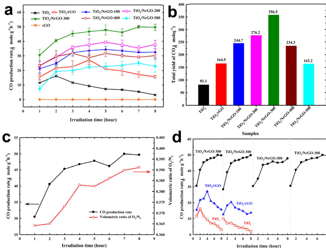
Fig. 4 (a) CO production rate via photocatalytic reduction of CO 2 with respect to irradiation time, and (b) total yield of CO under visible light irradiation using rGO, TiO 2 and TiO 2 /NrGO-X. (c) Rate of CO production and the volumetric ratio of O 2 /N 2 over TiO 2 /NrGO-300 for the CO 2 photocatalytic reduction rate through four consecutive cycles. Reproduced with permission from ref. 80, copyright 2017, Elsevier Ltd.
