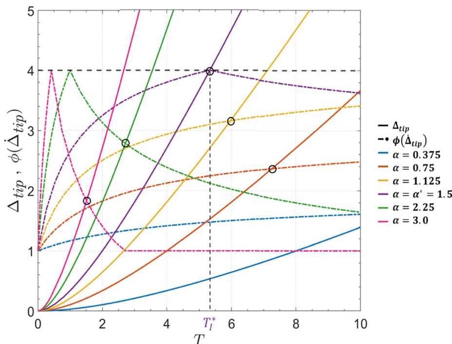
Fig. 4 Illustration of theory using (25a–c). The functions in (22), i.e., \Delta_{tip}(T) = (\sqrt{\beta^2 + \alpha T} - \beta)^2 (solid lines) and \phi(\dot{\Delta}_{tip}) = \phi\left(\left(1 - \frac{\beta}{\sqrt{\beta^2 + \alpha T}}\right)\alpha\right) (dash-dot lines) are plotted against normalized time T for 6 different normalized loading rates \alpha . The intersection of these curves, indicated by a circle, gives the initiation time T_l . (For \alpha = 0.375 , the initiation time T_l exceeds beyond the maximum plotted time of 10 and is therefore not displayed.) The curves are generated using \beta = \beta_0 = 1 , \phi_{max} = 4 , and \eta_{max} = 1 . For this case, the critical loading rate is \alpha^* = 1.5 . Consistent with theory, initiation occurs on the ascending/descending branch for \alpha < \alpha^*/\alpha > \alpha^* respectively.
