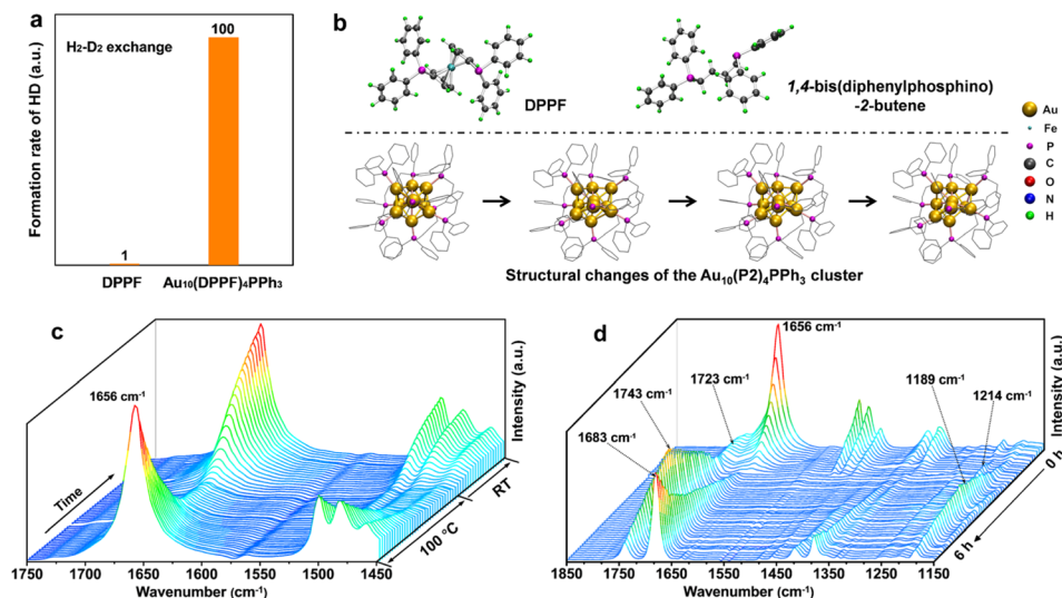
Fig. 4 (a) The normalized HD formation rate during the \text{H}_2\text{-D}_2 exchange reaction for the \text{Au}_{10}(\text{DPPF})_4\text{PPh}_3 cluster and the DPPF ligand, respectively. (b) Ligand substitution calculations of the \text{Au}_{10} cluster. The upper panel shows the structures of the DPPF ligand (left) and the simplified P2 ligand (right). The lower panel shows the structural changes of the \text{Au}_{10}(\text{P}2)_4\text{PPh}_3 cluster during optimizations (from left to right). (c) Time-resolved in situ FTIR spectra obtained from the reaction of pyrrolidine and \text{CO}_2 performed in the high-pressure liquid cell system without the catalyst. (d) Time-resolved in situ FTIR spectra corresponding to reaction intermediate species formed in the high-pressure liquid cell during the pyrrolidine hydroformylation reaction with \text{CO}_2 and \text{H}_2 catalysed by \text{Au}_{10} clusters.
