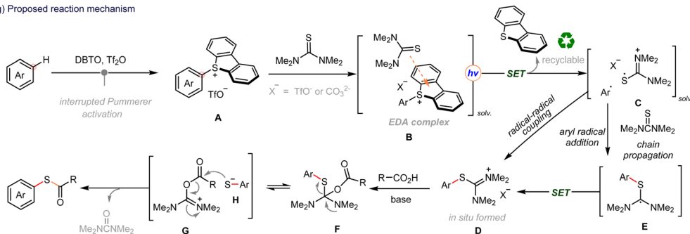
Scheme 3 Mechanistic studies.
