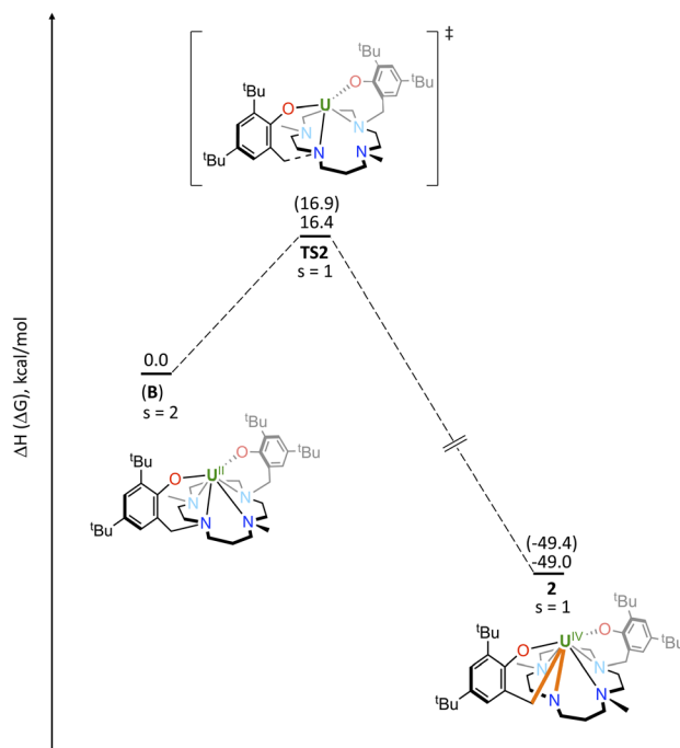
Fig. 7 Computed enthalpy profile (Gibbs free energy between brackets) at room temperature for the formation of complex 2 from intermediate B . The energies are given in \text{kcal mol}^{-1} . S stands for the total spin state of each intermediate.
