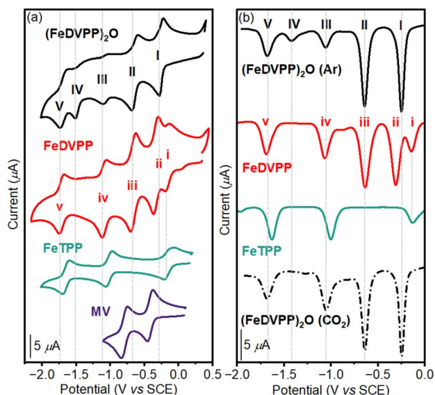
Fig. 1 (a) Cyclic voltammograms of 0.25 mM (\text{FeDVPP})_2\text{O} (black), 0.5 mM \text{FeDVPP} (red), 0.5 mM \text{FeTPP} (green), and 0.5 mM MV (purple) in DMF with 0.1 M [\text{Bu}_4\text{N}]\text{PF}_6 under Ar at 100 mV s -1 scan rate. (b) Differential pulse voltammograms of (\text{FeDVPP})_2\text{O} (black), \text{FeDVPP} (red) and \text{FeTPP} (green) in Ar, and (\text{FeDVPP})_2\text{O} in \text{CO}_2 (dash dot) [E step: 4 mV, amplitude: 50 mV, pulse width: 60 ms, sampling width: 20 ms, and pulse period: 500 ms].
