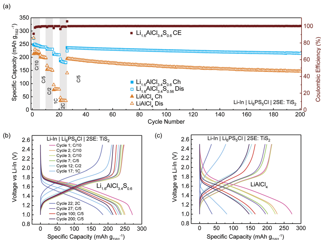
Fig. 5 Galvanostatic cycling of 2SE: \text{TiS}_2 catholyte with argyrodite \text{Li}_6\text{PS}_5\text{Cl} as the separator. (a) Rate performance of \text{Li-In}|\text{Li}_6\text{PS}_5\text{Cl}|2\text{SE}:\text{TiS}_2 cell (SE = \text{LiAlCl}_4 or \text{Li}_{1.6}\text{AlCl}_{3.4}\text{S}_{0.6} ) followed by long-term cycling at C/5, where C = 239\text{ mA h g}^{-1} . Voltage profile of cycle 1 along with the 2nd cycles of each C-rate for a (b) \text{Li-In}|\text{Li}_6\text{PS}_5\text{Cl}|2(\text{Li}_{1.6}\text{AlCl}_{3.4}\text{S}_{0.6}):\text{TiS}_2 cell and (c) \text{Li-In}|\text{Li}_6\text{PS}_5\text{Cl}|2(\text{LiAlCl}_4):\text{TiS}_2 cell.
