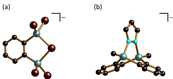
Fig. 4 Molecular structures in the solid state: (a) [\text{nBu}_4\text{N}][3] ; (b) [\text{K}(\text{thf})_{1.5}][1 \cdot (\mu\text{-pz})] . Counter cations and H atoms omitted for clarity. C: black, Br: brown, Al: turquoise, N: cyan.
