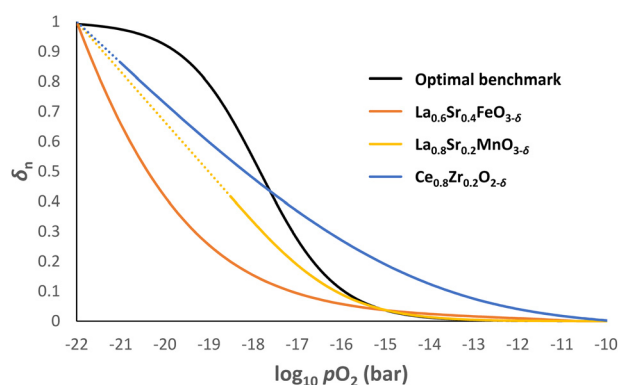
Fig. 8 \delta vs. \log_{10} p_{\text{O}_2} profiles for \text{La}_{0.6}\text{Sr}_{0.4}\text{FeO}_{3-\delta} , \text{La}_{0.8}\text{Sr}_{0.2}\text{MnO}_{3-\delta} and \text{Ce}_{0.8}\text{Zr}_{0.2}\text{O}_{2-\delta} at 1093 K using data from literature. 26,29,32 The optimal \delta - p_{\text{O}_2} relationship is also given as a benchmark. The dotted lines for \text{La}_{0.8}\text{Sr}_{0.2}\text{MnO}_{3-\delta} and \text{Ce}_{0.8}\text{Zr}_{0.2}\text{O}_{2-\delta} indicate extrapolation of the data if no decomposition were to occur.
