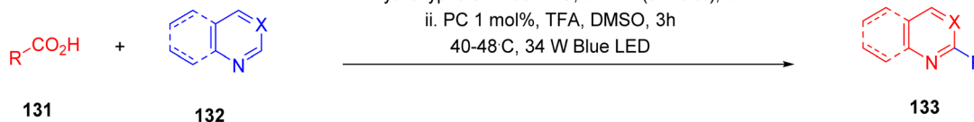
Fig. 63 Minisci reaction in the use of carboxylic acids in the presence of NAPs. 247
