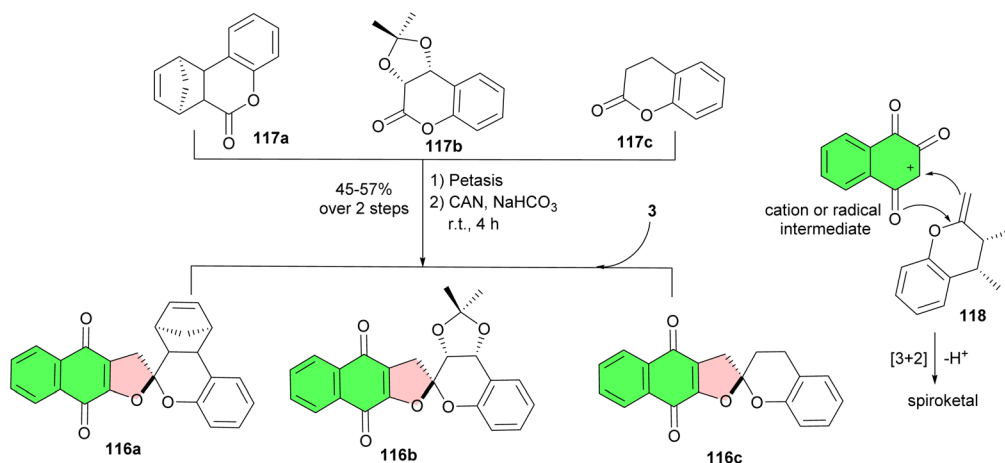
Scheme 31 Synthesis of naphthoquinone spiroketals 116 by diastereoselective oxidative [3 + 2] cycloaddition.
