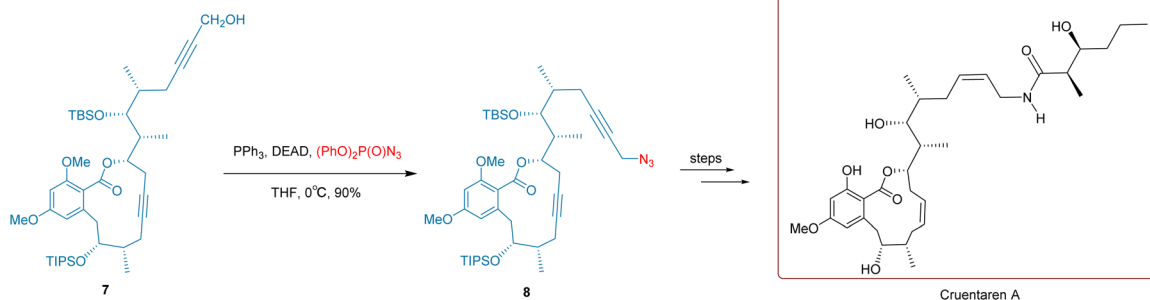
Scheme 5 Maier's synthesis of cruentaren A.
