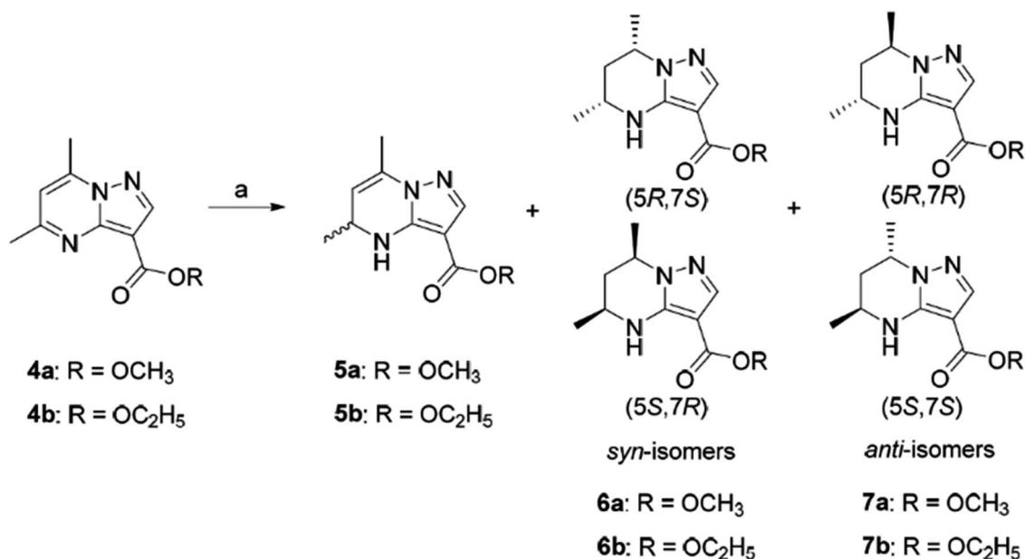
Scheme 27 Dearomatization of 5,7-dimethylpyrazolo[1,5- a ]pyrimidine-3-carboxylate. Reagents and conditions: (a) NaBH 4 , ROH, R 4 Na, R = CH 3 , and C 2 H 5 . 107
