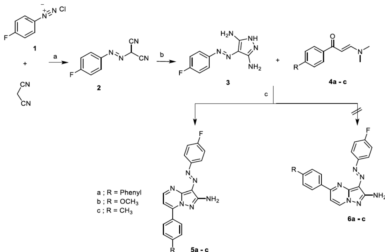
Scheme 28 The preparation of 3-((4-fluorophenyl)diazenyl)-7-(4-substituted phenyl)pyrazolo[1,5- a ]pyrimidin-2-amine 5a–c . Reagents and condition: (a) sodium acetate/EtOH, stirring for 30 min/cooling. (b) NH 2 NH 2 ·H 2 O/EtOH, reflux 6 h. (c) GL acetic acid, reflux 7 h.
