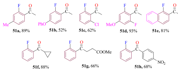
Scheme 23 Palladium-catalyzed ortho C–H fluorination of aromatic ketones.
