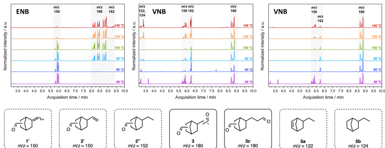
Fig. 2 Stacked GC chromatograms from hydroformylation reactions of ENB (1) and VNB (2) at different temperatures after three hours; reaction conditions: (left) 24.96 mmol ENB (1), 0.10 mol% [\text{Rh}(\text{COD})_2\text{BF}_4] , 0.31 mol% Alkanox®, \text{CO}/\text{H}_2 = 1/1 , 50 bar, 40–140 °C, (PhMe, 1 M). (middle) 24.96 mmol VNB (2), 0.10 mol% [\text{Rh}(\text{COD})_2\text{BF}_4] , 0.11 mol% Oxophos®, \text{CO}/\text{H}_2 = 1/1 , 50 bar, 40–140 °C, (PhMe, 1 M). (right) 24.96 mmol VNB (2), 0.10 mol% [\text{Rh}(\text{COD})_2\text{BF}_4] , 0.11 mol% Oxophos®, \text{CO}/\text{H}_2 = 3/2 , 50 bar, 40–140 °C, (PhMe, 1 M). Byproducts: aldehydes 1' ( m/z = 150 ) result from ENB (1) hydroformylation; aldehydes 2' ( m/z = 150 ) and 2'' ( m/z = 152 ) result from VNB (2) hydroformylation; hydrogenated compounds 5a ( m/z = 122 ) and 5b ( m/z = 124 ) emerge as byproducts from VNB (2) hydroformylation with a syngas ratio of \text{CO}/\text{H}_2 = 1/1 .
