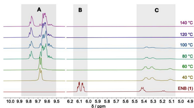
Fig. 1 Stacked ^1\text{H} NMR spectra from hydroformylation reactions of ENB (1) at different temperatures after three hours using Alkanox® as the ligand; reaction conditions: 0.10 mol% [\text{Rh}(\text{COD})_2\text{BF}_4] , 0.35 mol% Alkanox®, \text{CO}/\text{H}_2 = 1/1 , 50 bar, 40–140 °C, 3 h, (PhMe, 1 M). (A): characteristic resonances of aldehyde groups. (B): characteristic resonances of endocyclic double bonds. (C): characteristic resonances of cis/trans exocyclic double bonds.
