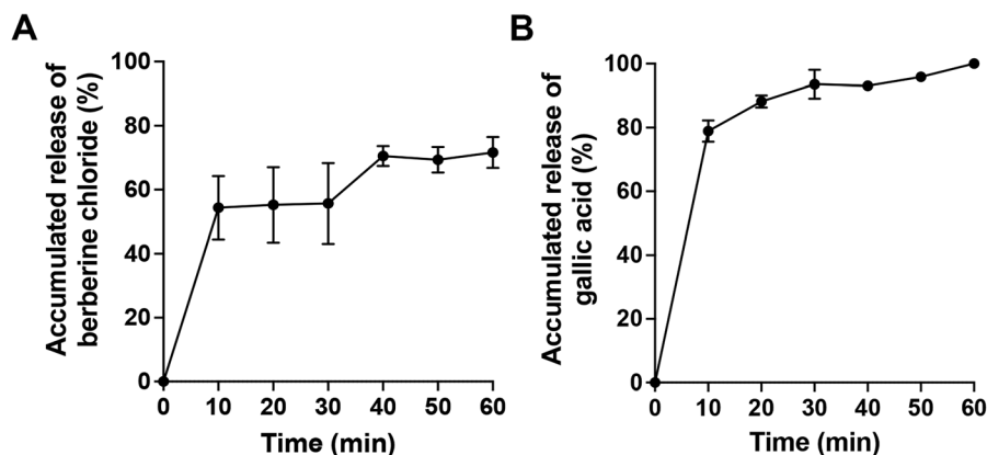
Fig. 3 Drug release profiles of SDF–PCL/PEO nanofiber meshes. (A) Cumulative drug release curve for berberine chloride from SDF–PCL/PEO nanofiber meshes. (B) Cumulative drug release curve for gallic acid from SDF–PCL/PEO nanofiber meshes. Bars represent the mean \pm SEM of 3 independent assays.
