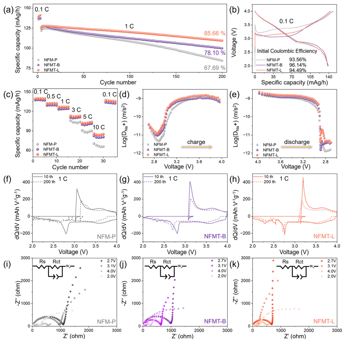
Fig. 6 (a) Cycling performance; (b) the first charge/discharge curve at 12 \text{ mA h g}^{-1} ; (c) rate performance; (d and e) GITT-calculated diffusion coefficients ( D_{Na^+} ) of NFM-P, NFMT-B and NFMT-L; (f–h) dQ/dV curves after the 10th and 200th cycles; and (i–k) in situ EIS Nyquist plots at different potentials of NFM-P/NFMT-B/NFMT-L.
