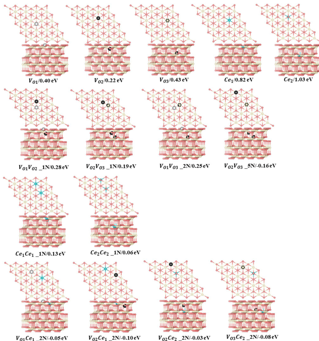
Fig. 2 15 primary features predicted by statistical learning and their energies, with structures depicted in the unrelaxed state. Ce 4+ , Ce 3+ , oxygen atoms, and surface oxygen vacancy are depicted in white, blue, pink, and light gray, respectively. Subsurface and third oxygen layer vacancies are depicted in black.
