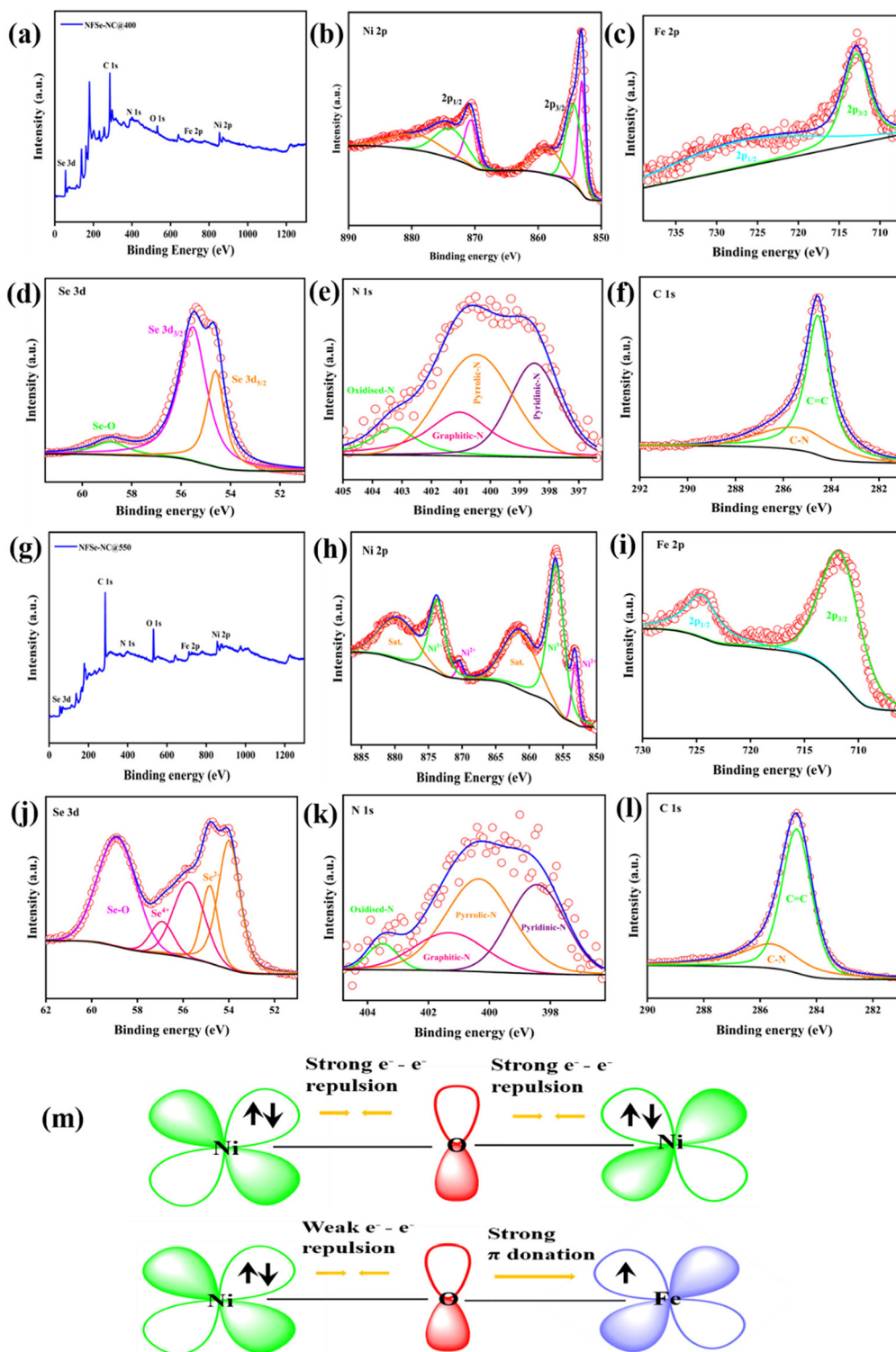
Fig. 5 High-resolution XPS spectra of (a and g) survey scan (b and h) Ni 2p, (c and i) Fe 2p, (d and j) Se 3d, (e and k) N 1s, (f and l) C 1s of Ni x Fe 1-x Se 2 -NC@400 and Ni 3-x FeSe 4 -NC@550, (m) schematic representation of electronic coupling of Ni–O–Fe in Ni x Fe 1-x Se 2 -NC@400.
