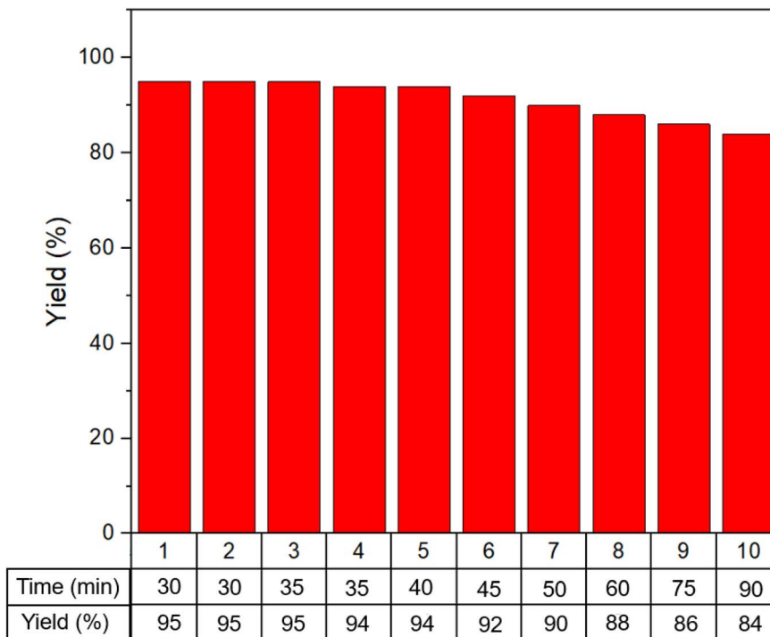
Fig. 10 Recoverability and reusability of \text{Fe}_3\text{O}_4@\text{MCM-41}@UiO-66/\text{SB-Pd} .
