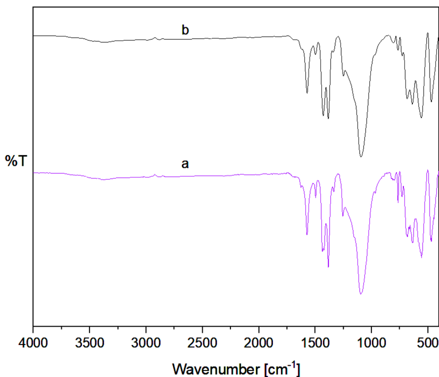
Fig. 11 FTIR spectra of (a) fresh and (b) recovered \text{Fe}_3\text{O}_4@\text{MCM-41}@UiO-66/\text{SB-Pd} catalyst.
