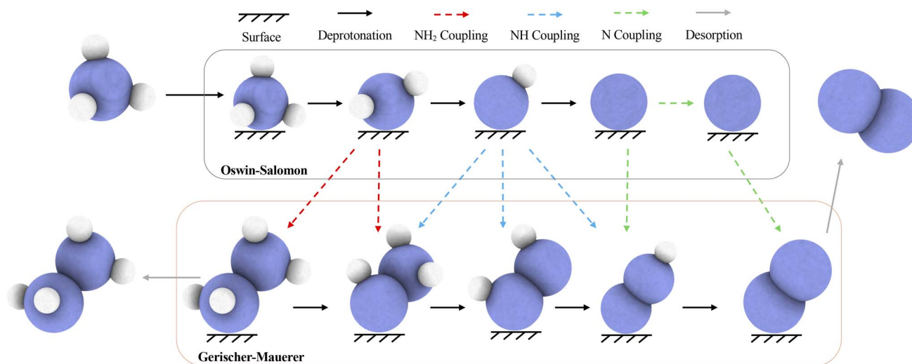
Fig. 1 AOR mechanisms toward N 2 and N 2 H 4 formation. Blue and white spheres are nitrogen and hydrogen atoms, respectively. The Oswin-Salomon mechanism and the Gerischer-Mauerer mechanism are outlined by a black and orange box, respectively.
