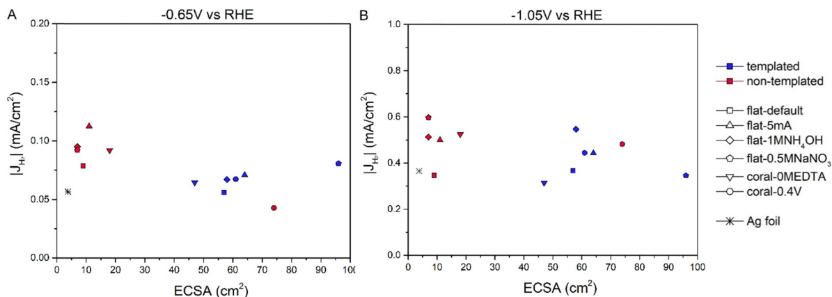
Fig. 8 Partial current densities to H_2 for both the template-based porous (blue) and non-templated equivalent (red) samples (n)t-flat-default, (n)t-flat-5mA, (n)t-flat-1MNH 4 OH, (n)t-flat-0.5MNaNO 3 , (n)t-coral-0MEDTA and (n)t-coral-0.4V at (A) -0.65 V vs. RHE and (B) -1.05 V vs. RHE plotted versus the ECSA.
